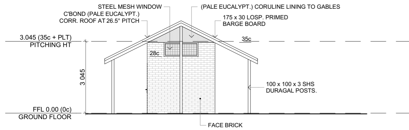
ELEVATION E-2 1:100 A2
